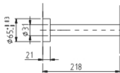
Spindle Hole
