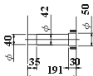
Spindle Hole
